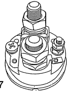
AL 3109 Replacing Bosch Servicing 0331 303 133- 142 2339 303 201,-205 3 terminals Crimp style
