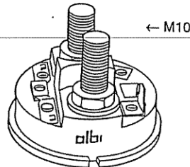
AL 3064 Replacing Bosch Servicing 0331402535 Insulated return Cap 3 terminals. Contact AL 3058
