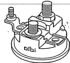
AL 3019 Replacing Mitsubishi Servicing M371 x 66571 PMGR Startes 3 terminals Contact AL 3014
