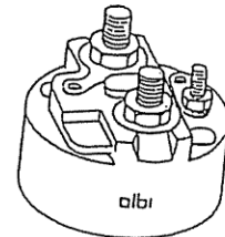
AL 272 Replacing Ducellier Servicing 583098, 681726 3 terminals
