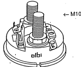
AL 3063 Replacing Bosch Servicing 0331402012 4 terminals Insulated return Cap 24 v Contact AL 3058
