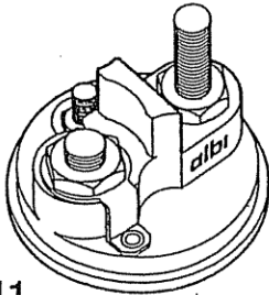
AL 3111 Replacing Bosch Servicing Modified cap for 2339304008 Solenoids Citroen, Peugeot (3 terminals)
